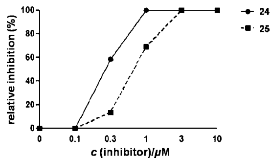
Figure 5. Relative TGase inhibition percentage of moenomycin A ( 24 ) and its analogue 25 via HPLC analysis with substrate 7 .
