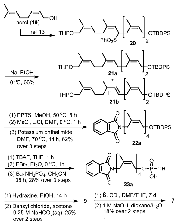
Scheme 2. Synthesis of the Probe Molecule 7 a
